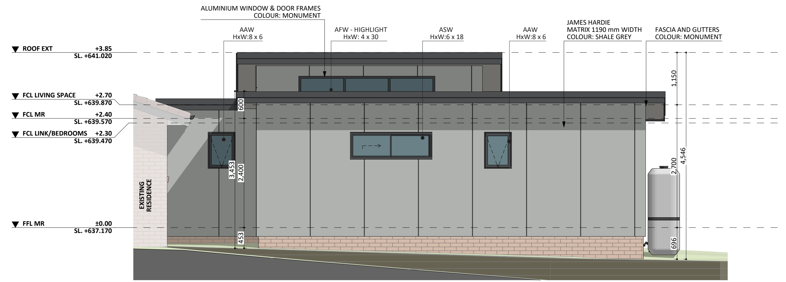
NORTH ELEV.
