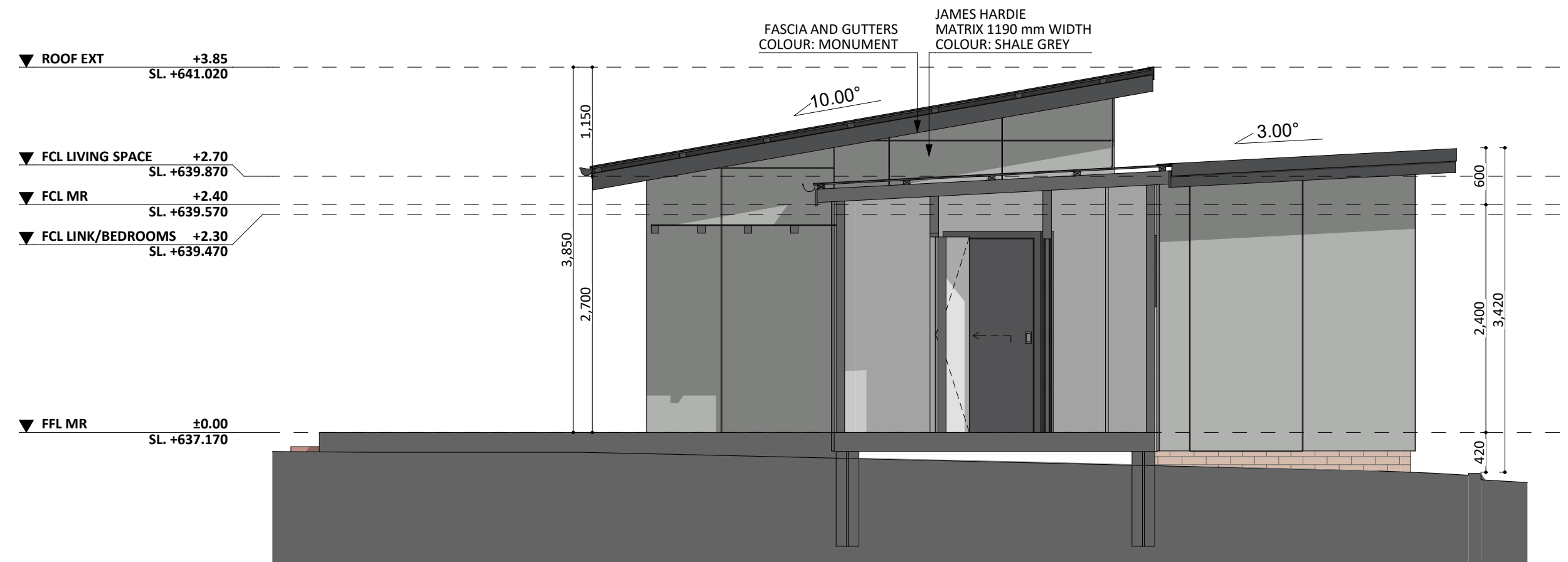
EAST ELEV.
