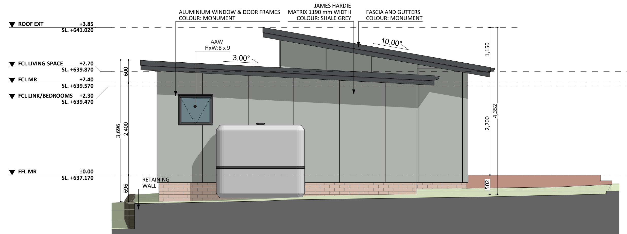
WEST ELEV.
