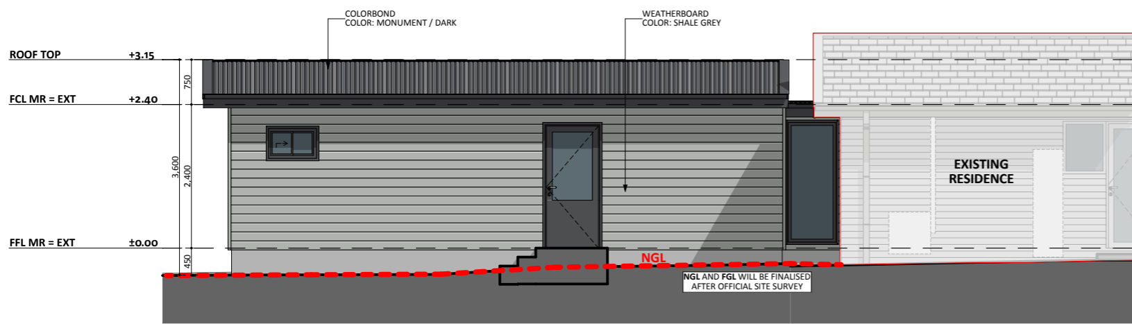
SOUTH ELEVATION - CD
