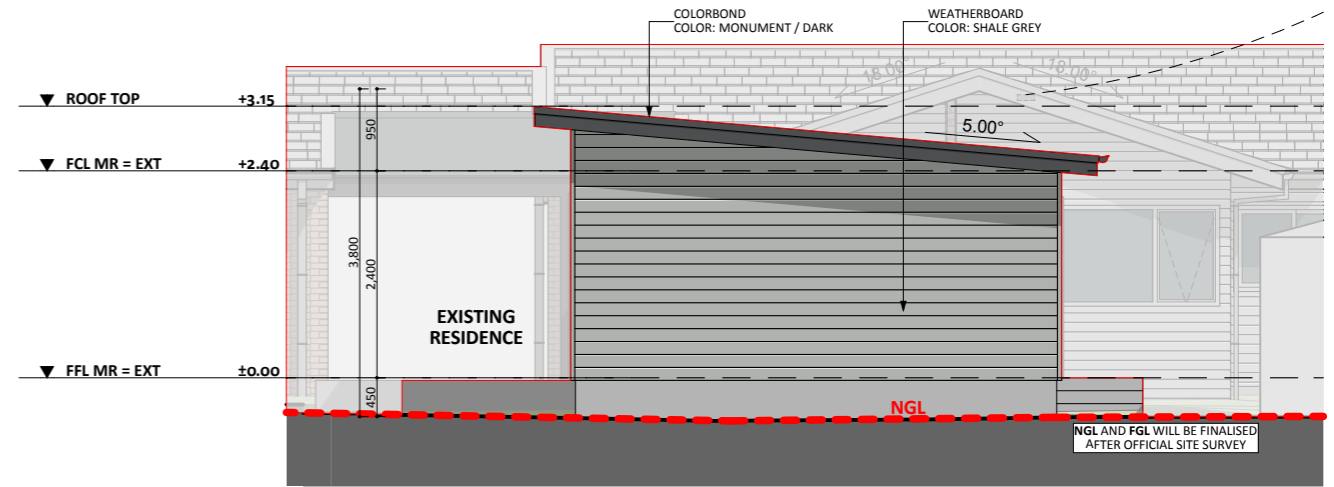
WEST ELEVATION - CD
