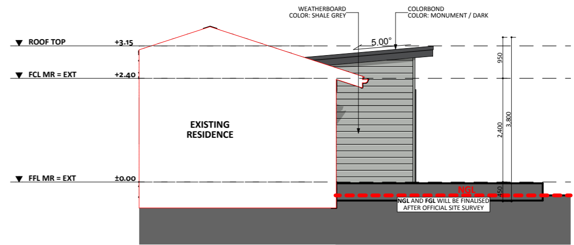
EAST ELEVATION - CD
