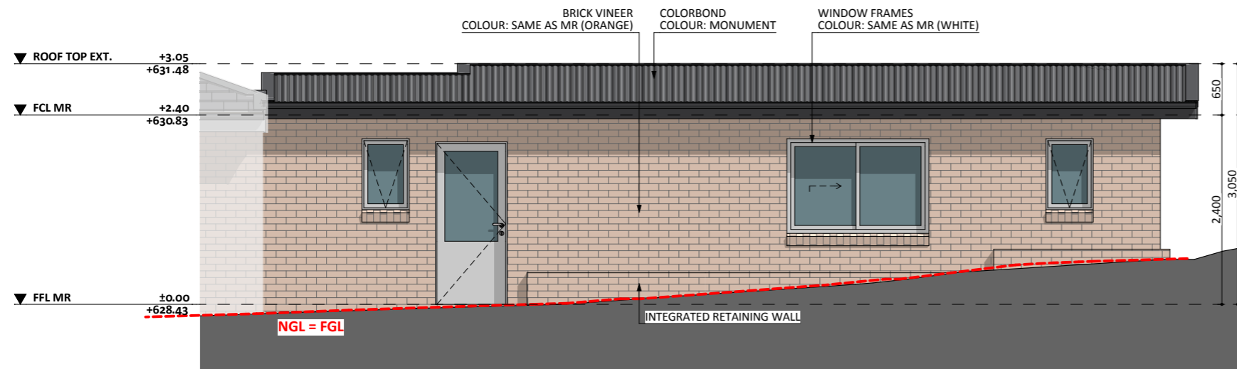
ELEVATION 03
