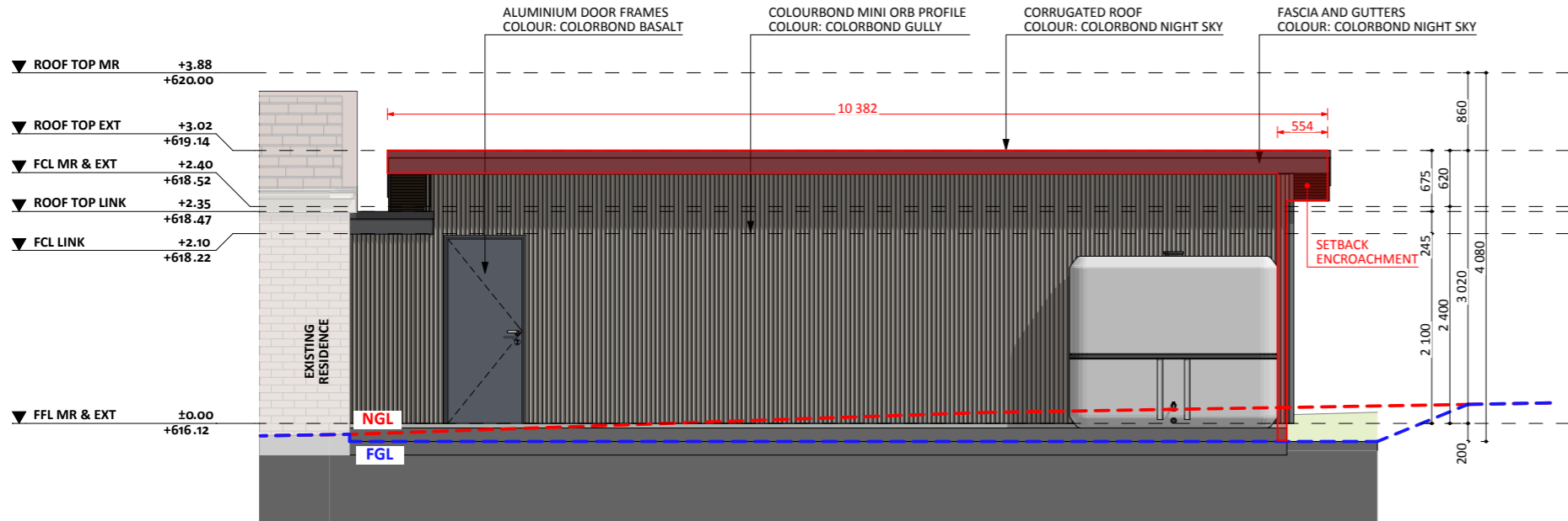
ELEVATION 03
