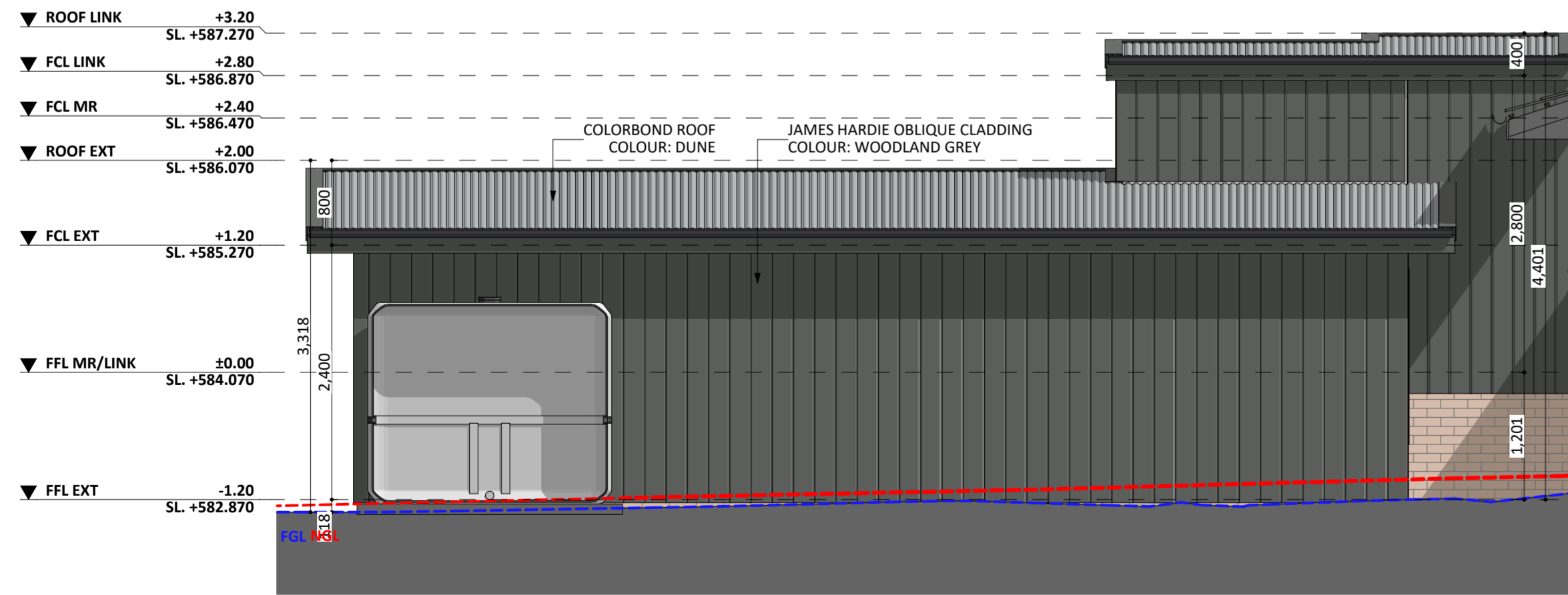
SOUTH ELEV.
