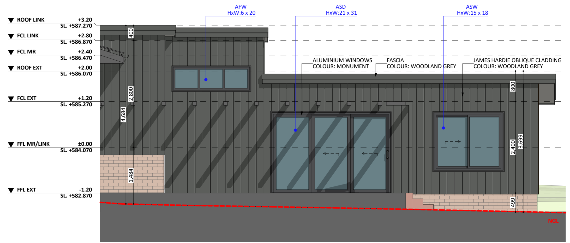
NORTH ELEV.
