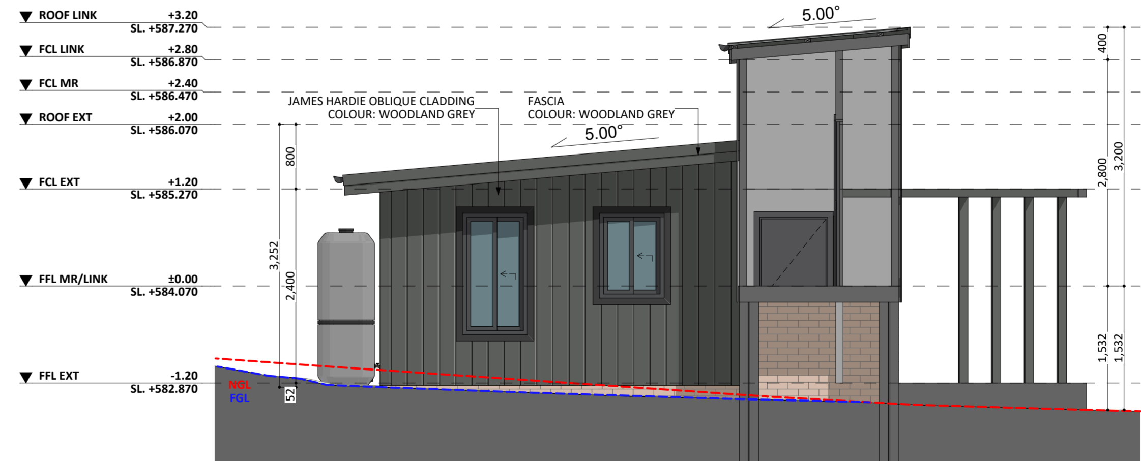
EAST ELEV.
