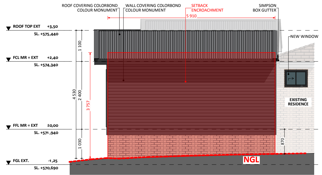
ELEVATION 03
