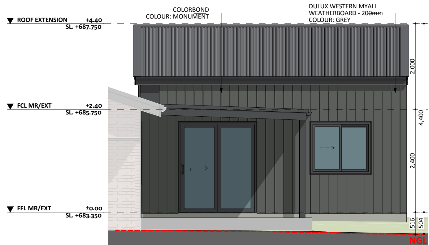
ELEVATION 03
