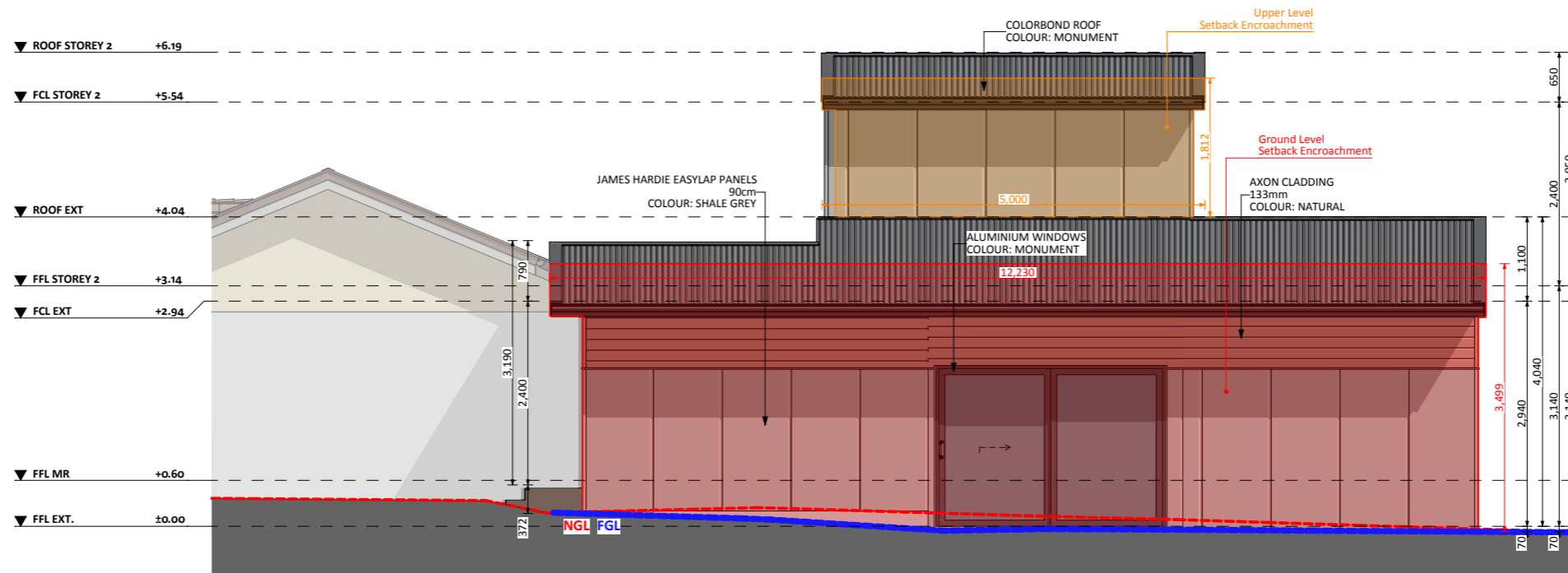
ELEVATION 03
