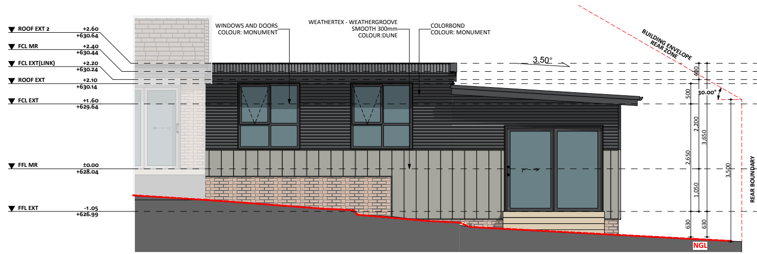
NORTH ELEV.
