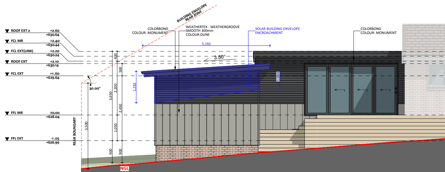
SOUTH ELEV.
