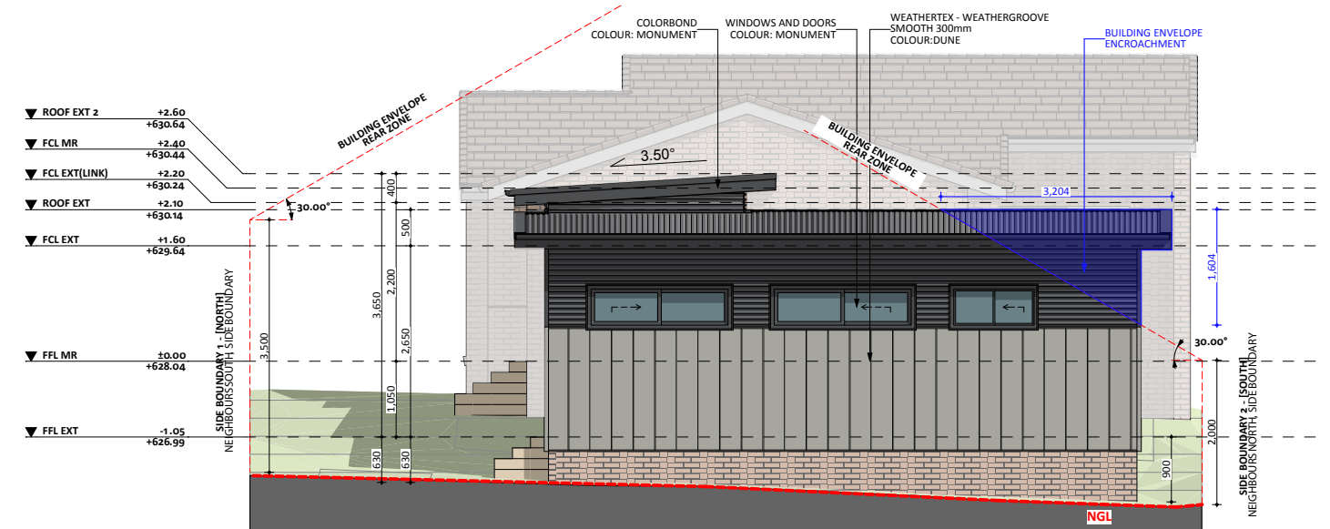
WEST ELEV.
