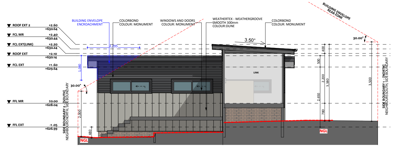
EAST ELEV.
