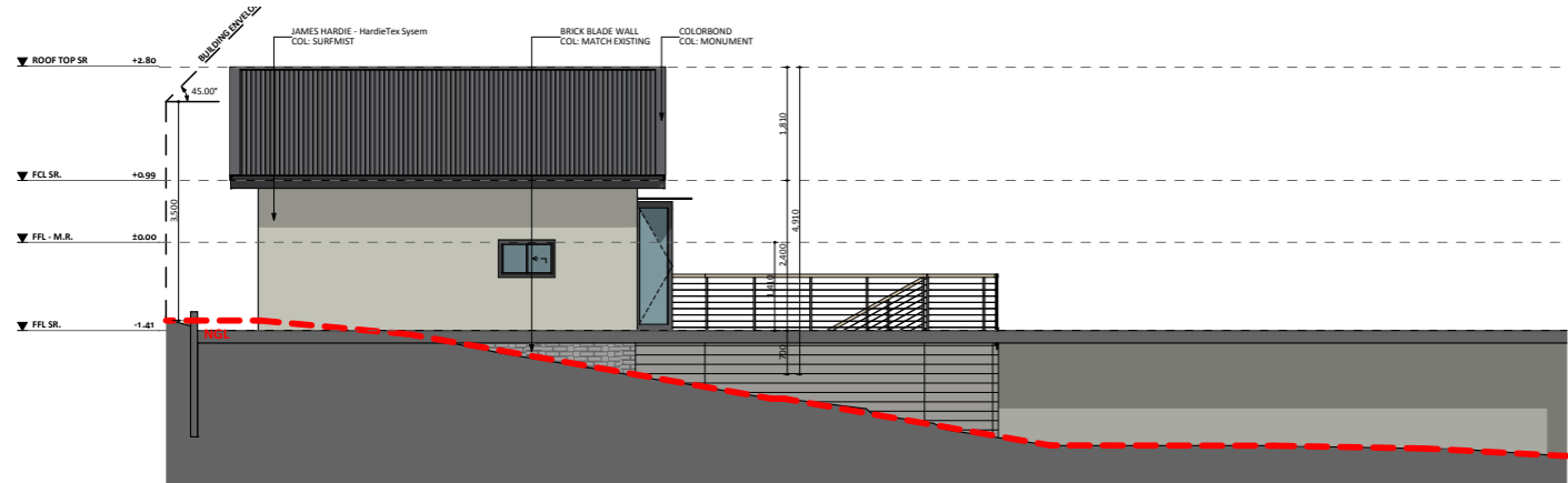
ELEVATION 03
