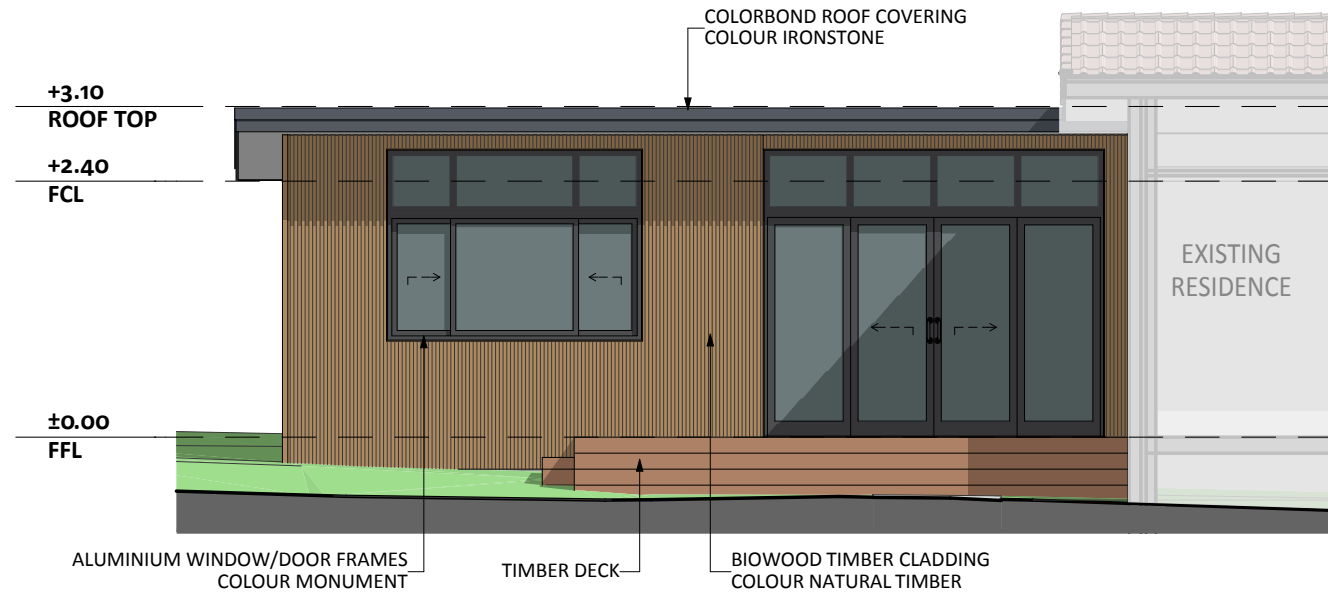
NORTH ELEVATION
