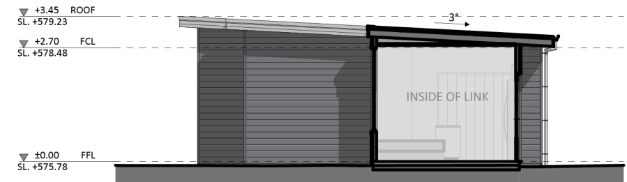
WEST ELEVATION
