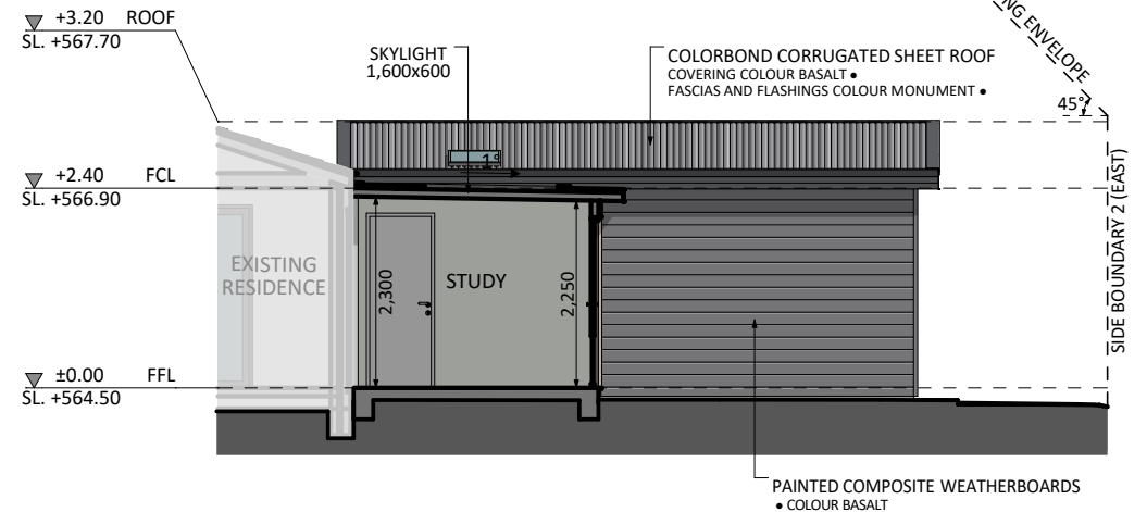
SOUTH ELEVATION
