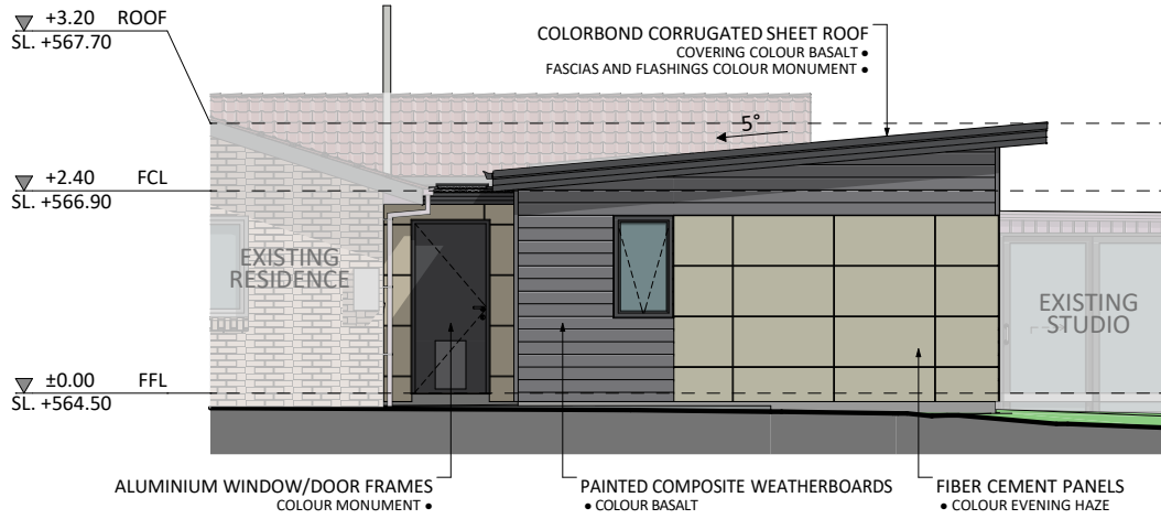
EAST ELEVATION
