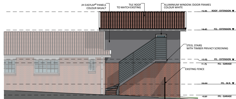
NORTH-WEST ELEVATION
