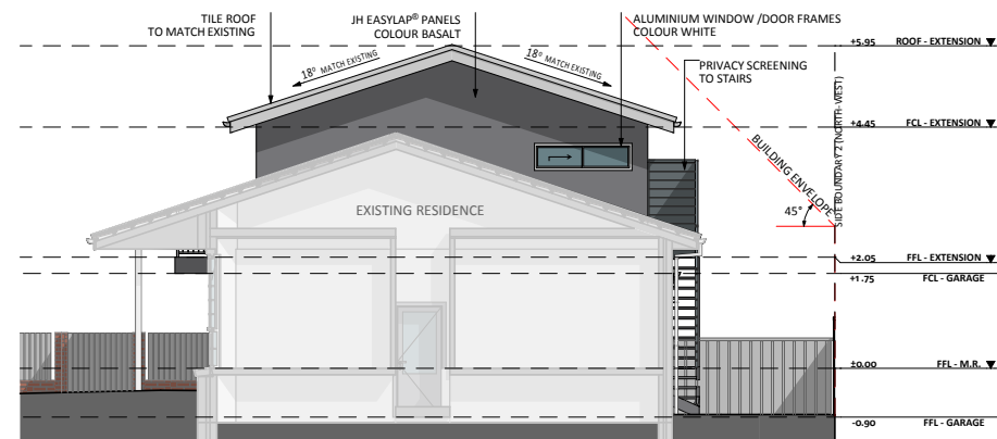
NORTH-EAST ELEVATION
