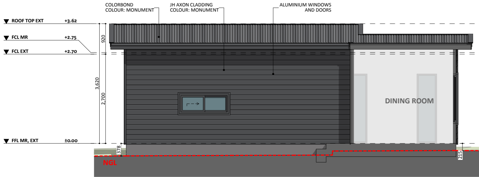
ELEVATION 03
