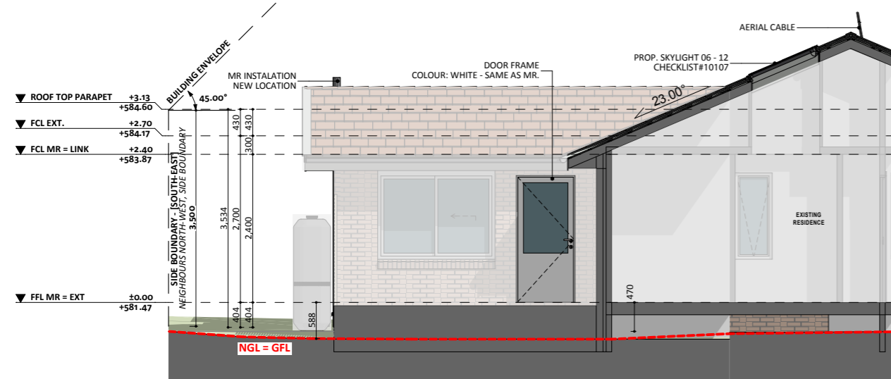
ELEVATION 03
